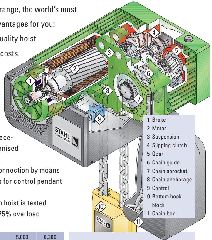
Chain hoist with hook suspension
