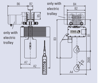
Chain hoist with trolley
